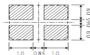
Land Pattern(REFERENCE)
