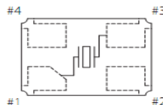
Land Pattern(REFERENCE)
